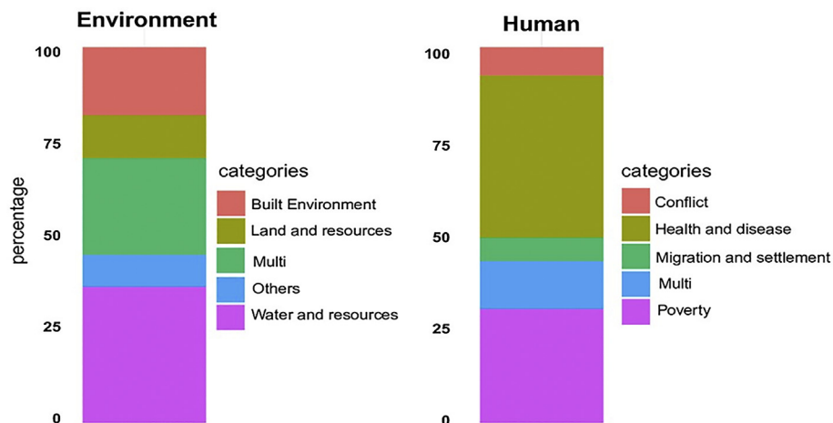
Figure 10. Summary of CC impact publications (1962–2019) in environment and human impact categories.
