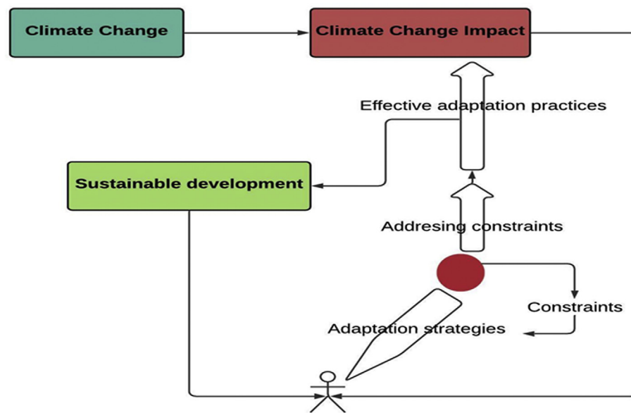
Figure 11. Conceptual diagram showing links between CC and sustainable development through effective adaptation by addressing the identified constraints (After Bizikova et al., 2007).
