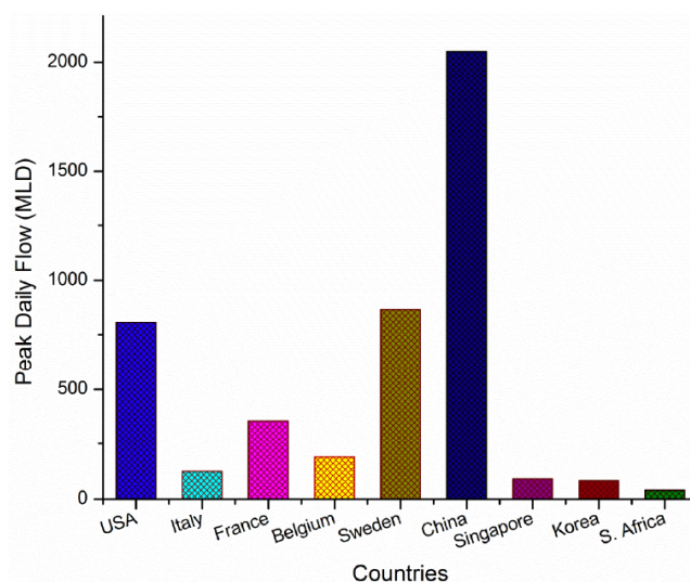
Figure 3: World's Largest MBR plants in mega liters per day [Sampled number of plant(s) in each country starting from USA include; 3, 1, 1, 1, 1, 13, 1, 1, in that order between year 2014 and 2017] (Source: The MBR Site [21]).
