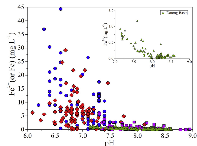
Fig. 7. Relationship between Fe 2+ (or dissolved Fe) concentrations and pH in high As groundwater (As > 10 μg L -1 ) from different countries or regions. Blue circles represent Cambodia and Vietnam (data from Rowland et al., 2008; Berg et al., 2008), red diamonds represent Bangladesh and West Bengal (India) (data from Nickson et al., 2000; Bhattacharya et al., 2009; Halim et al., 2009; Stüben et al., 2003), purple squares represent Inner Mongolia (China) (data from Guo et al., 2008, 2011), and olive triangle represent Datong (China) (data from Zhang et al., 2017; Xie et al., 2013a; Wang et al., 2014; and fraction of data from this survey). (For interpretation of the references to colour in this figure legend, the reader is referred to the Web version of this article.)
