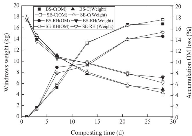
Fig. 2. Windrows weight characteristics and cumulative OM loss during composting process.
