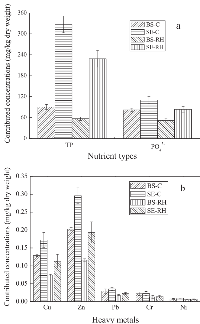
Fig. 6. The contributed concentrations of (a) potential nutrients retention about TP, \text{PO}_4^{3-} and (b) heavy metals immobilized for final composts.
