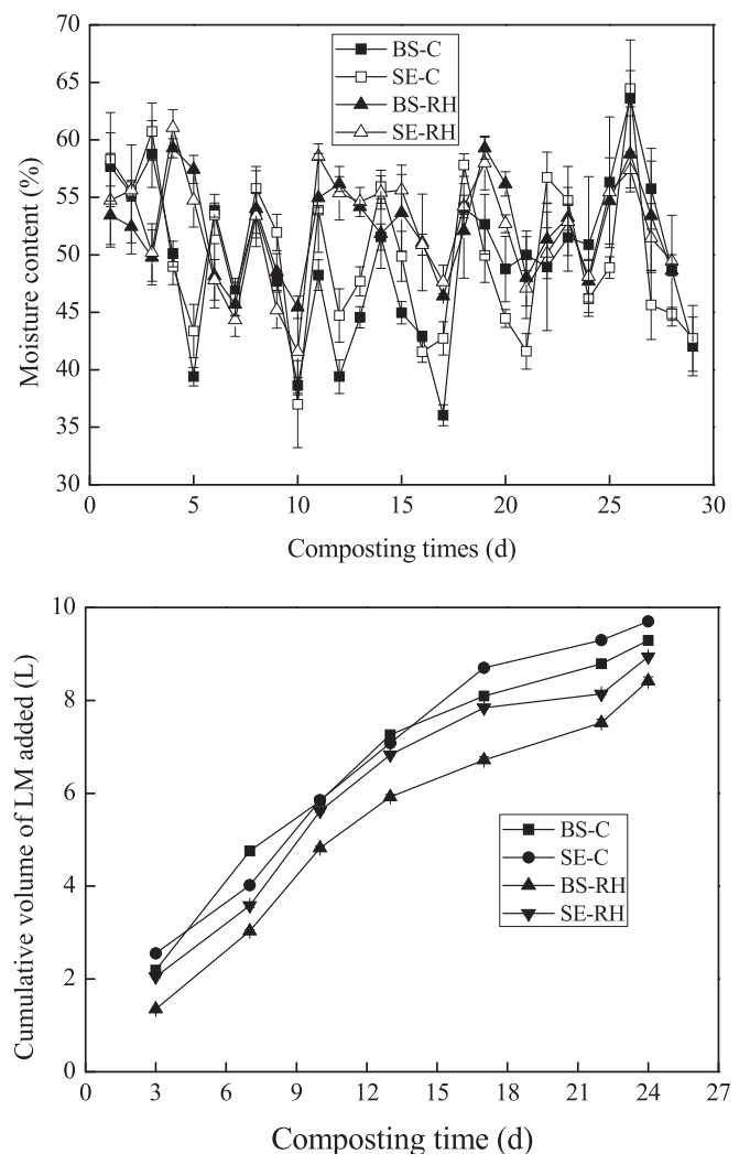
Fig. 3. Moisture content of different windrows and cumulative volumes of LM added during composting process.
