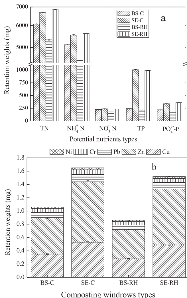
Fig. 5. The retention weights of (a) potential nutrients and (b) heavy metals.
