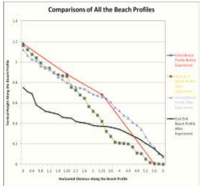
Figure 5. Comparison of beach profiles at different sections before and after the experiment
