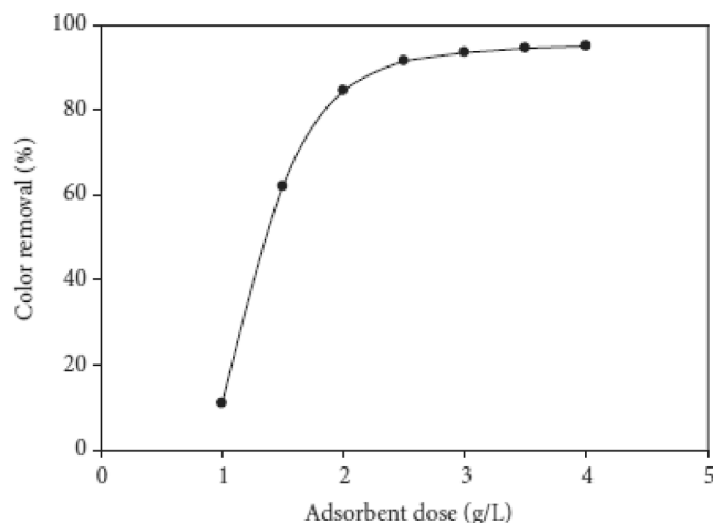
Fig. 3. Sugar cane stalk powder's effect as an adsorbent dosage on the color removal of Maxilon Red (El-Sayed et al., 2013).
