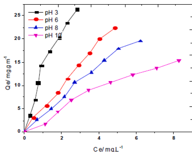
Fig. 1. Effect of pH on the adsorption of Maxilon Blue on the surface of Coconut shell (Aljeboree et al., 2020). (For interpretation of the references to color in this figure legend, the reader is referred to the web version of this article.)
