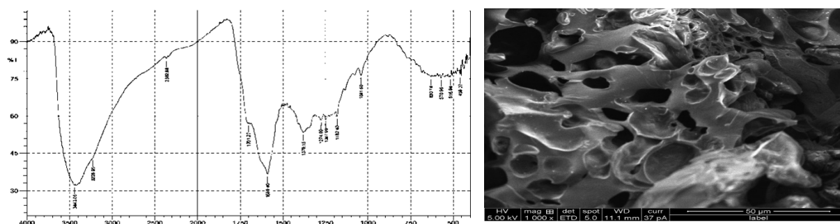
Figure 6. FTIR spectrum of Mlg (a), SEM image of Mlg (b).
