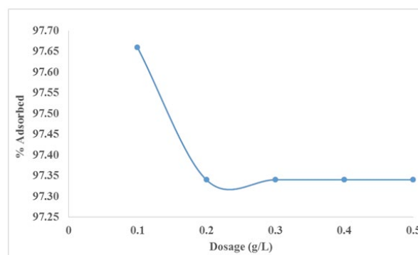
Figure 2. Adsorbent load effect on MG uptake onto MIg [Temperature (26 °C), pH (6.0) and agitation speed (130 rpm)] [n = 3, 0 ≤ SD ≤ 0.0027].
