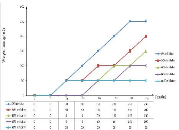
Figure.2 Weight loss-time curves of carbon steel in 0.1M HCl in the absence and presence of different concentrations of Cashew inhibitor
