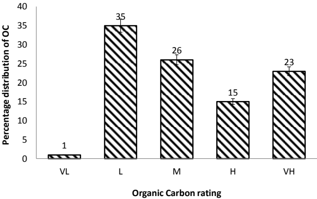
Fig. 6b: Percentage rating of organic carbon
