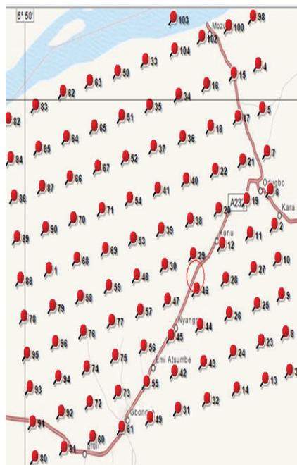
Fig. 3: Composite sampling points
