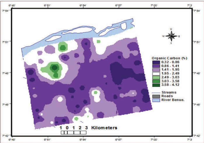
Fig. 6a: Spatial distribution of organic carbon
