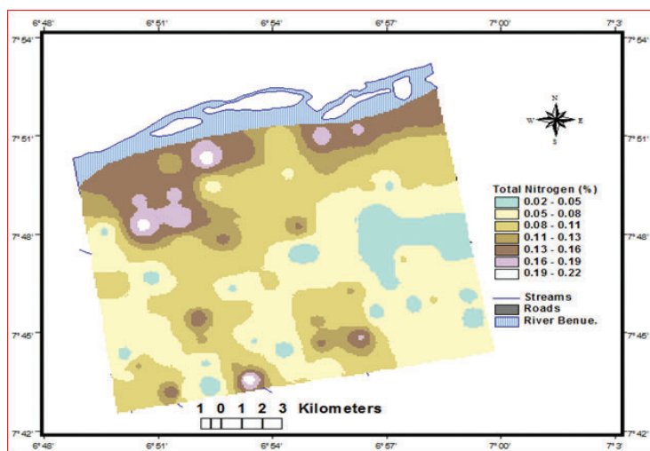
Fig. 7a: Spatial distribution of total nitrogen
