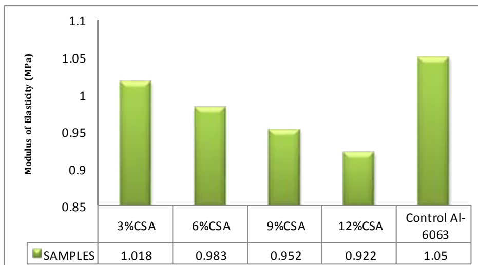
Figure 8. Shows the variation of Modulus of Elasticity for the control sample and reinforced AA6063/CSA composite
