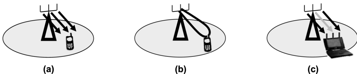
Figure 4. Benefits of multiple antennas: (a) diversity gain; (b) array gain; (c) spatial multiplexing gain
