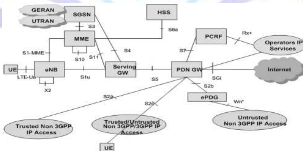
Figure 4: LTE system architecture [7]
