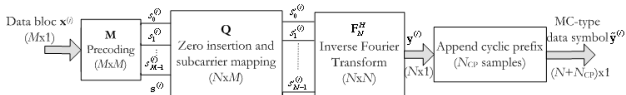
Figure 2: Baseband Structure of a Generalized Multi-Carrier Transmitter [4]
