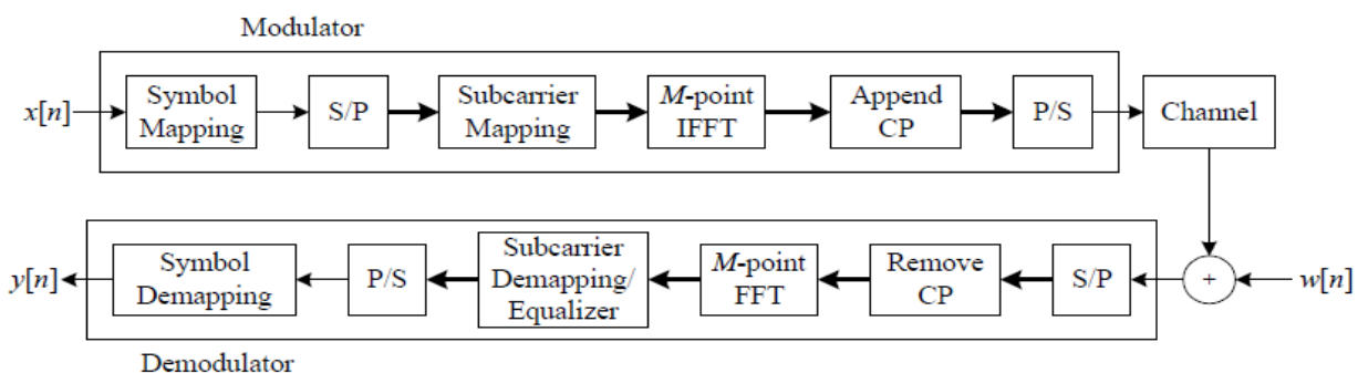
Figure 1: Block Diagram of OFDMA [10]
