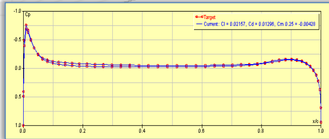
Figure 6: Pressure distribution
