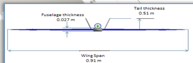
Figure 2: Front View
